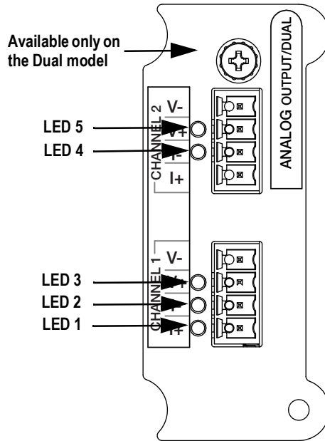
Figure 3. Analog Output Card Faceplate (Dual Analog Output Card)
