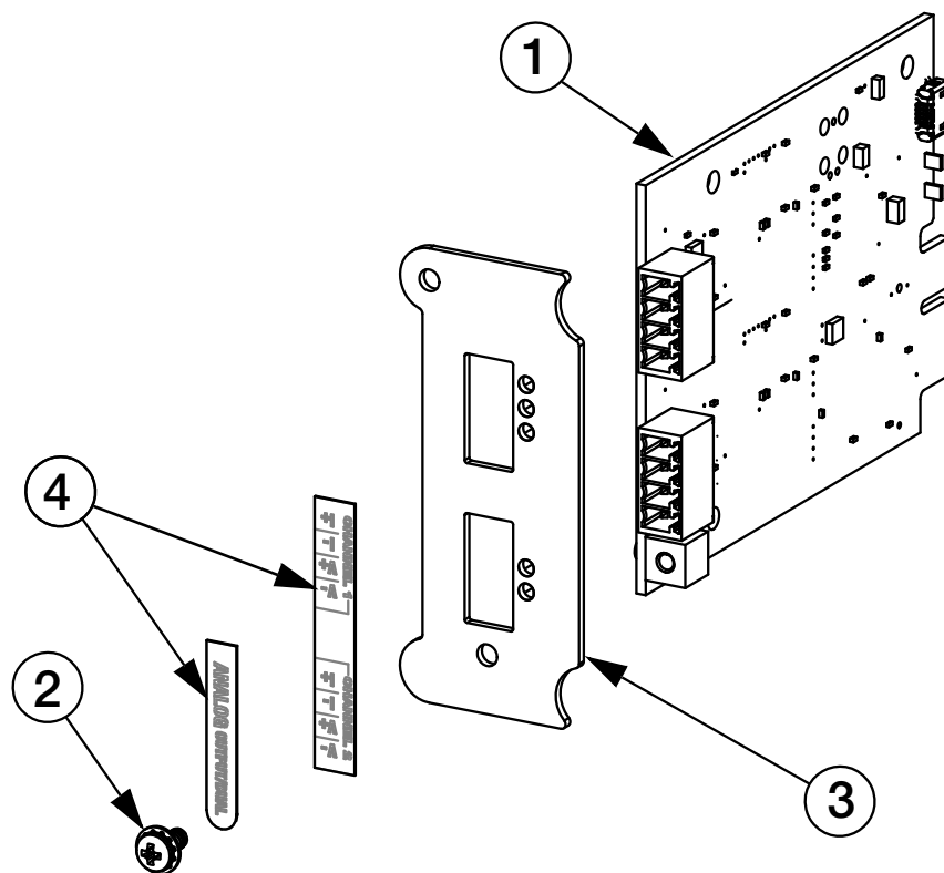
Figure 1. Dual Analog Output Card Kit
