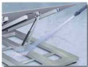
The rugged design incorporates 304 stainless steel construction and four welded seal load cells with PTFE cable designed for high temperatures and washdown areas.
