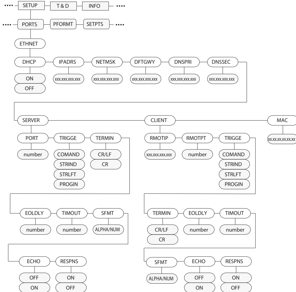
Illustration 3-13. Structure du menu Ethernet
