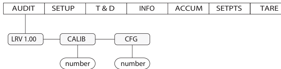
Illustration 3-3. Structure du menu Audit
