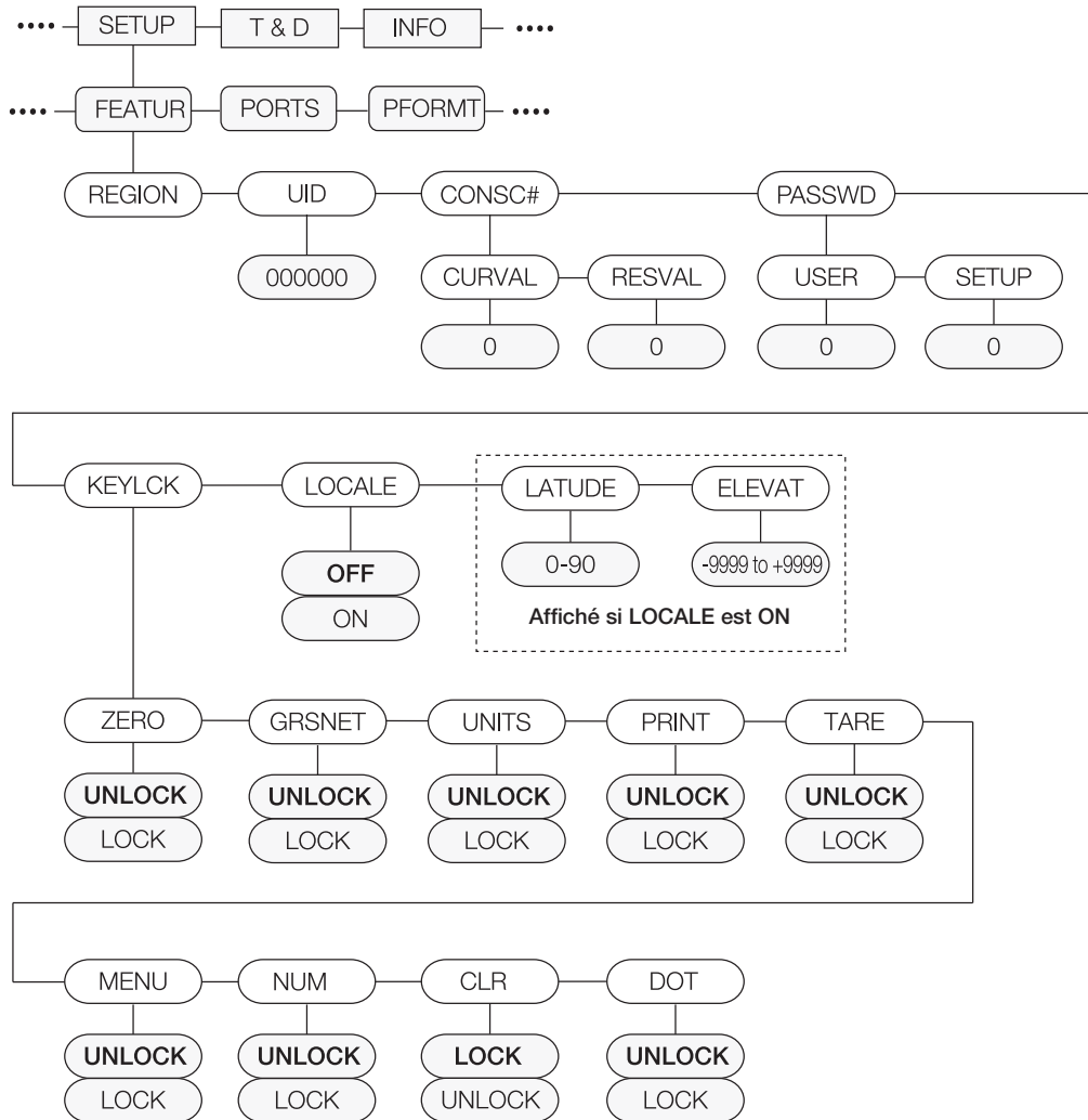
Illustration 3-9. Structure du menu Feature
