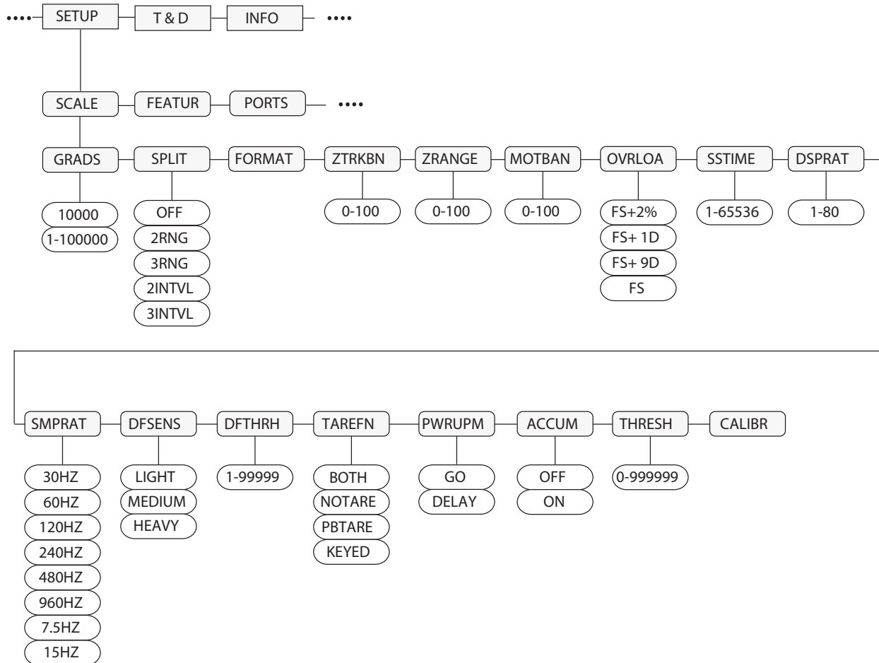
Illustration 3-5. Structure du menu Balance
