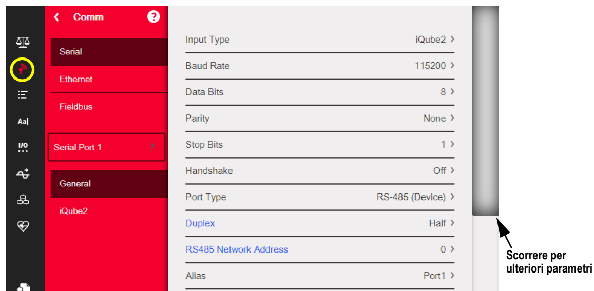
Figura 5-1. Menu Communications
