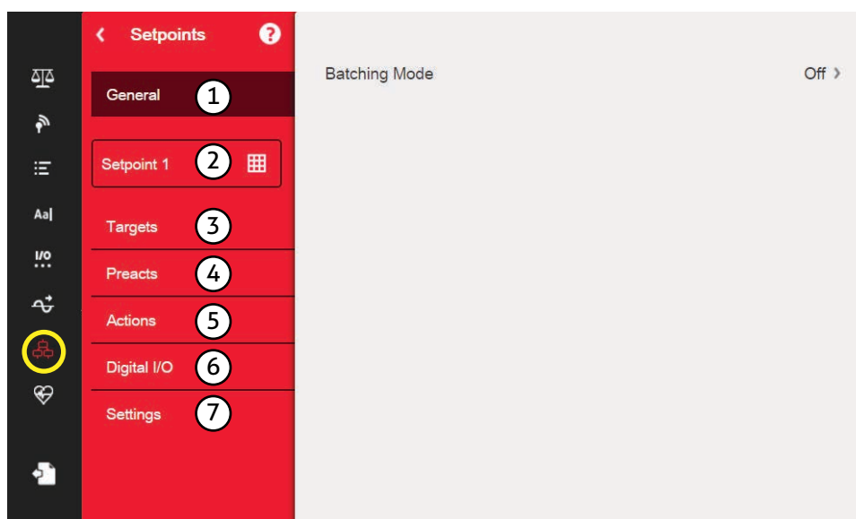
Figura 10-1. Menu Setpoints
