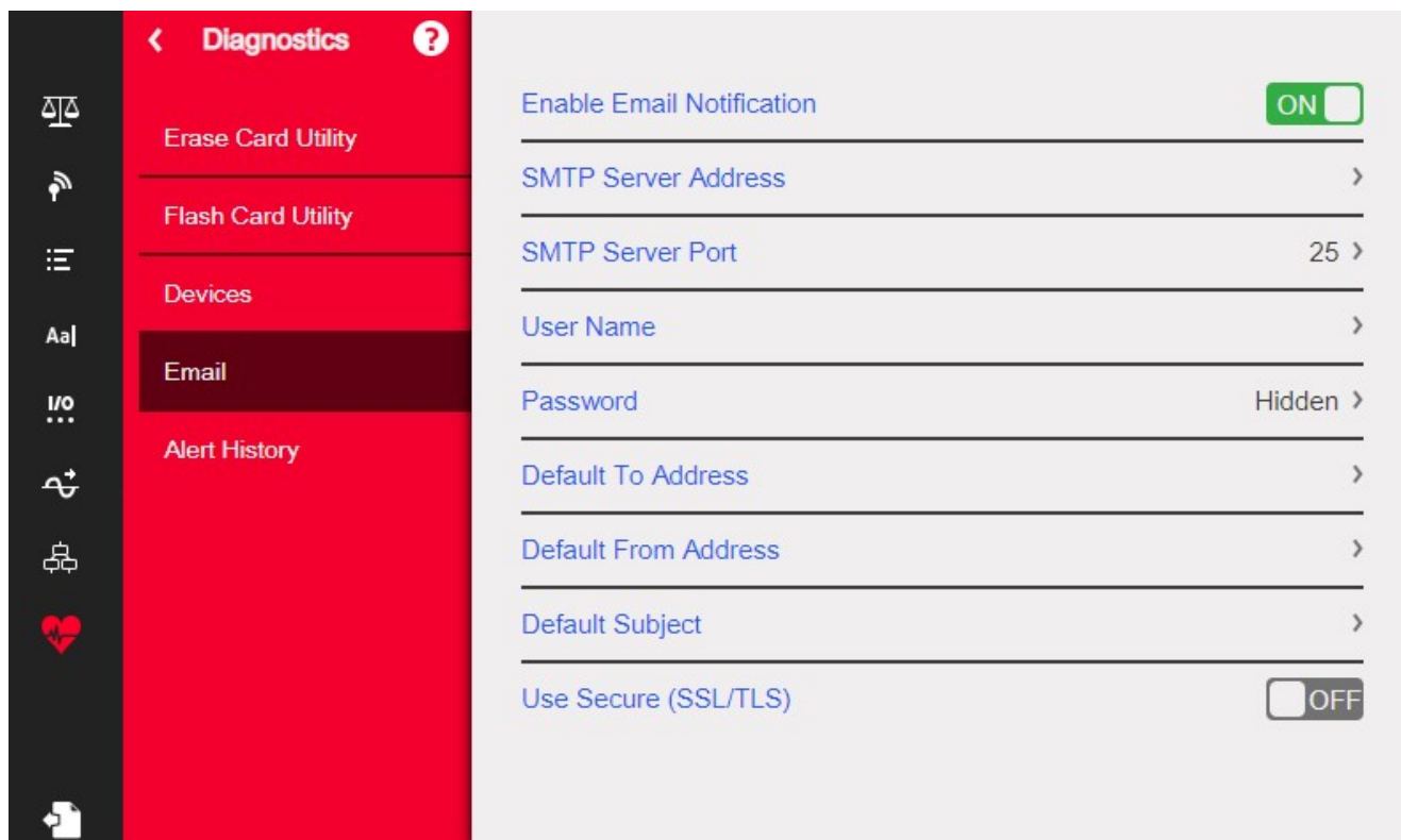
Figura 11-5. Menu Email
