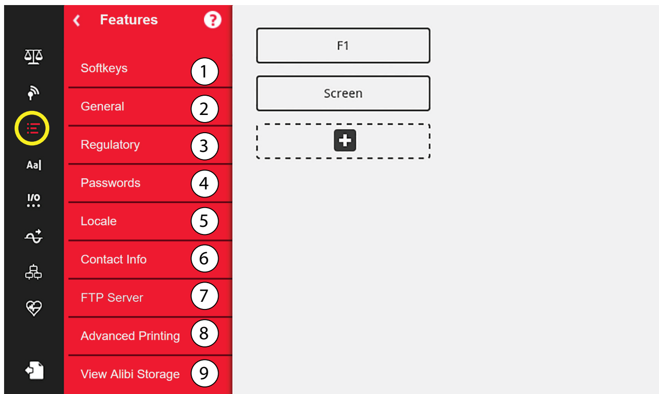
Figura 6-1. Menu Features
