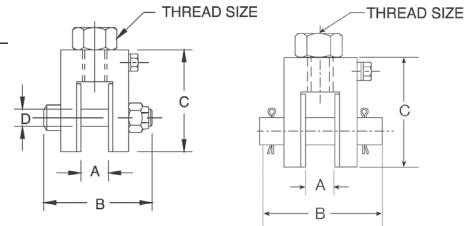
Clevis Mount with bolt
