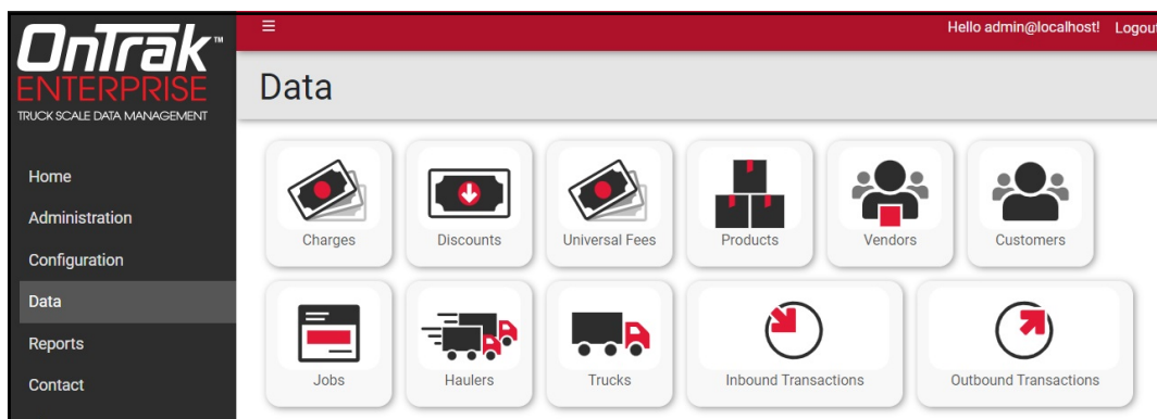
Figure 7-1. Data Page
