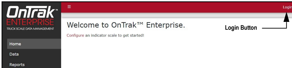
Figure 3-2. Login Button
