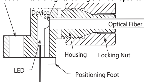
Figure 3. Fiber Optics Connector
