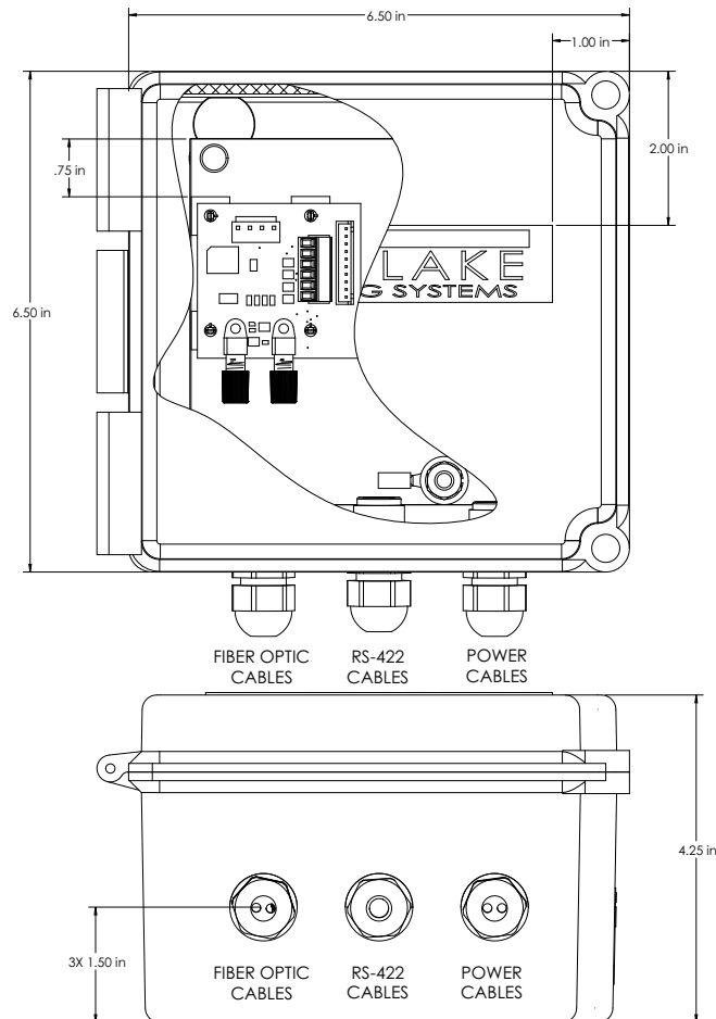
Figure 1. Fiber Optics to RS-422 Converter RFP Enclosure
