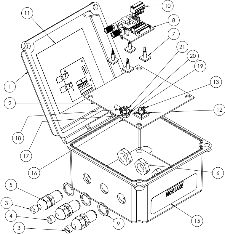
Figure 5. Replacement Parts
