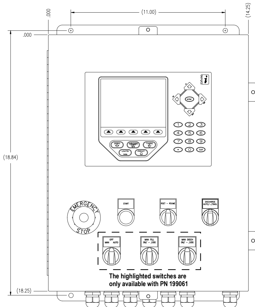
Figure 1-1. FlexWeigh System 102
