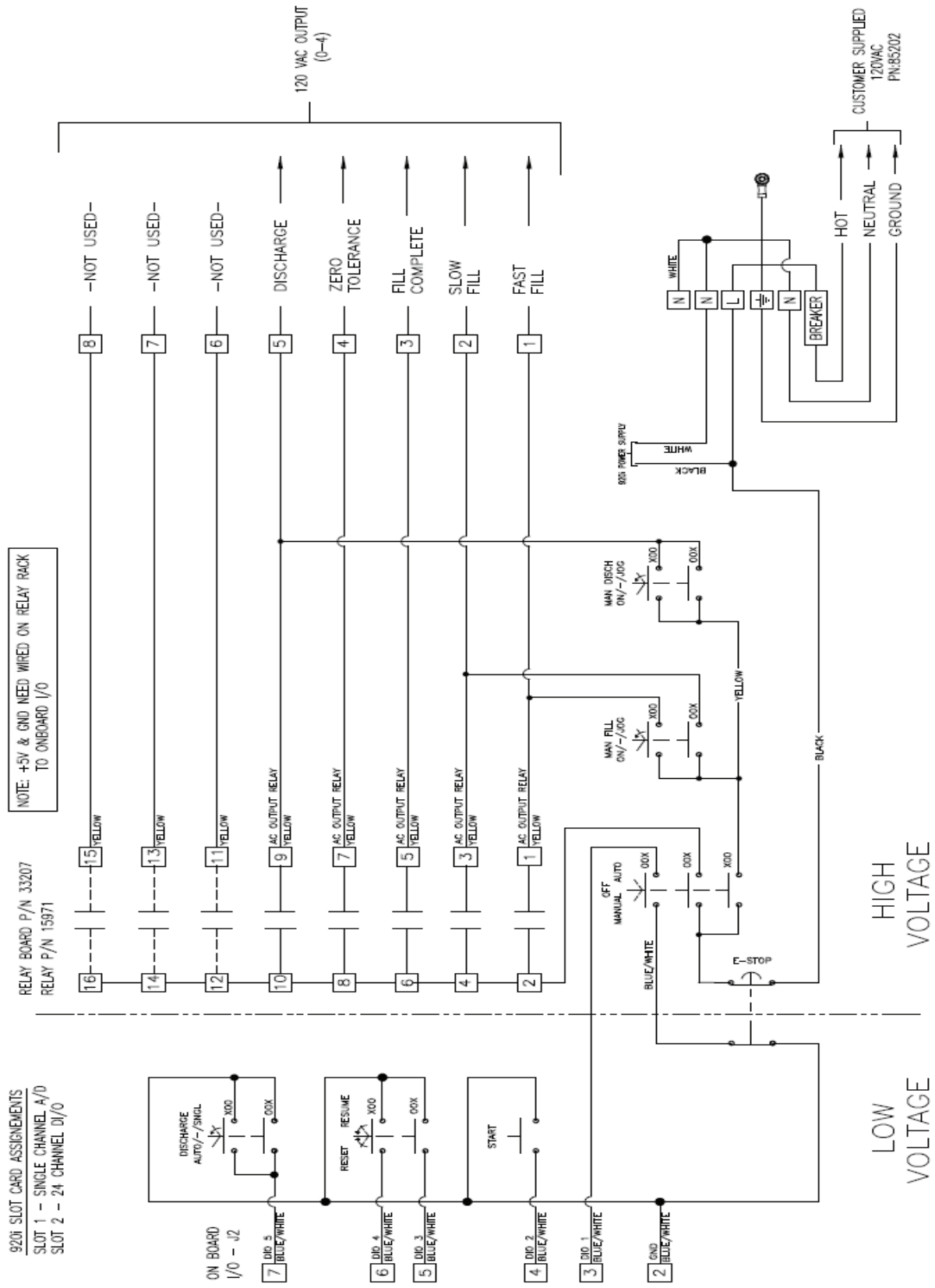
Figure 2-2. Block Wiring Diagram with Additional Controls
