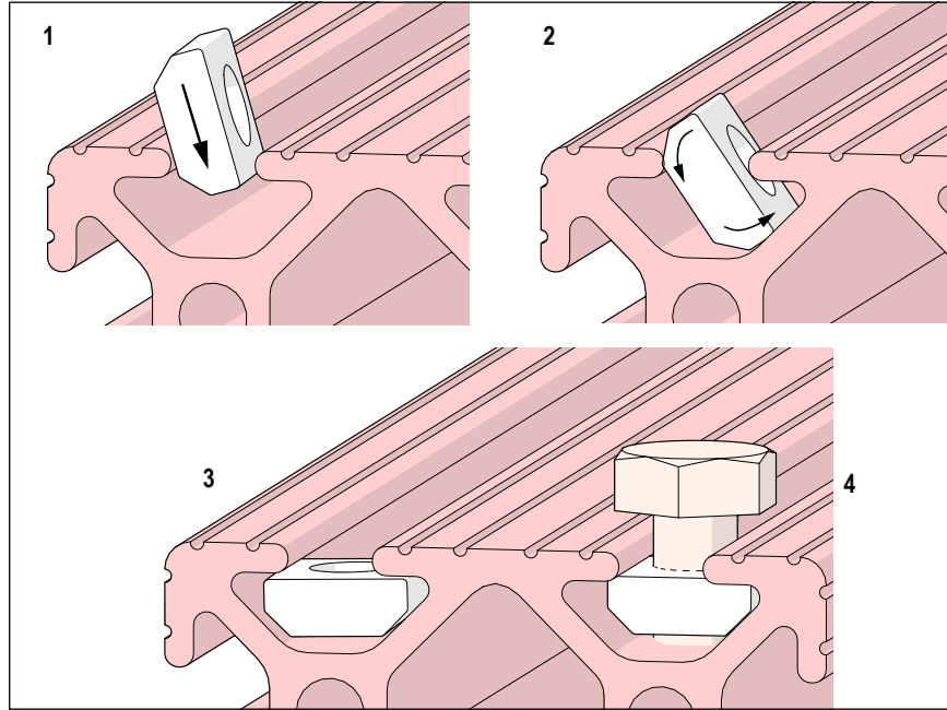
Figure 3-2. Roll-in T-bolts
