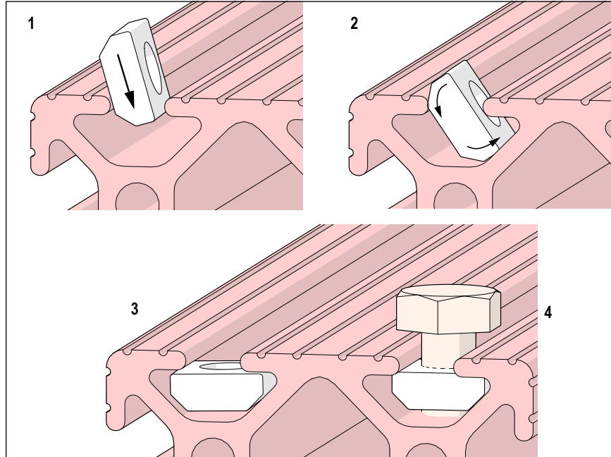
Figure 3-2. Roll-in T-bolts
